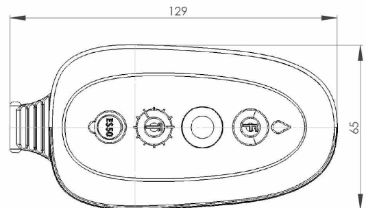
Basic Dimensions (mm)
